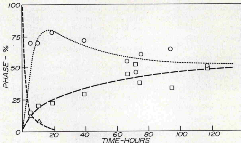
FIG. 3. The trend with time of the disappearance of anatase and of the slow crystallization of II. By difference, the amount of a short range order transition phase of \text{TiO}_2 is estimated. ( \triangle = anatase; \square = II; \circ = SRO).
